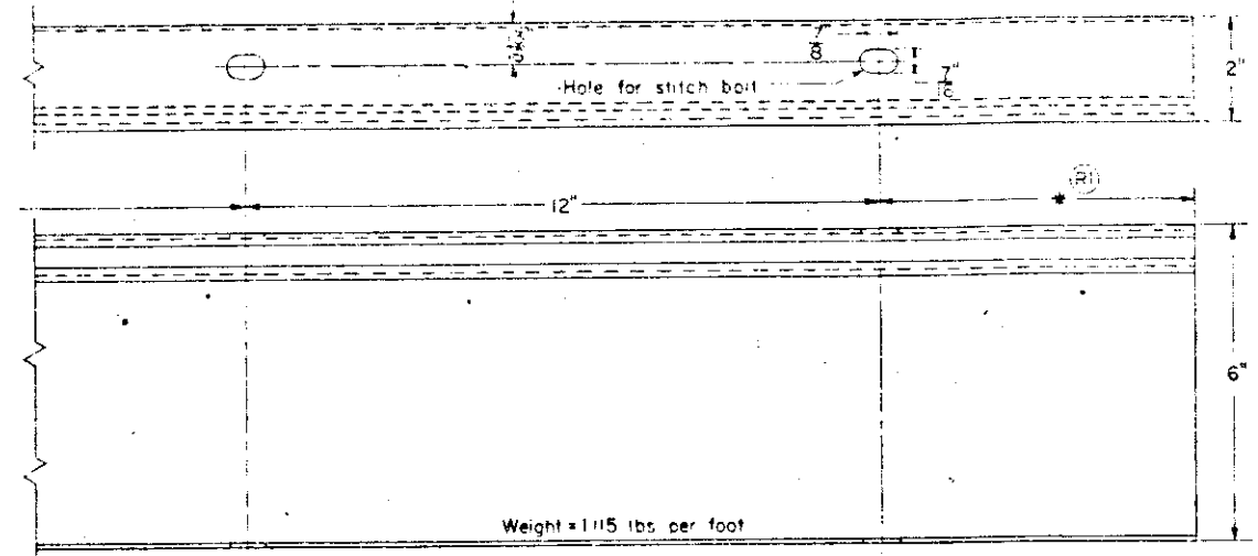
6" EXTRUDED ALUMINUM CHANNEL REAR VIEW
