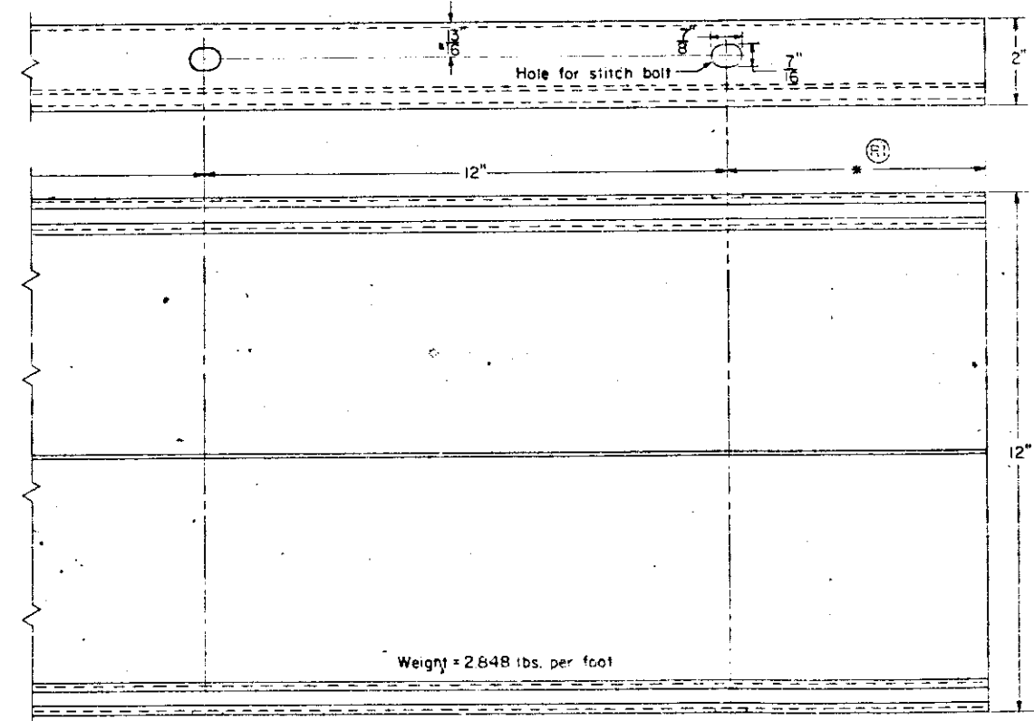
12" EXTRUDED ALUMINUM CHANNEL REAR VIEW
