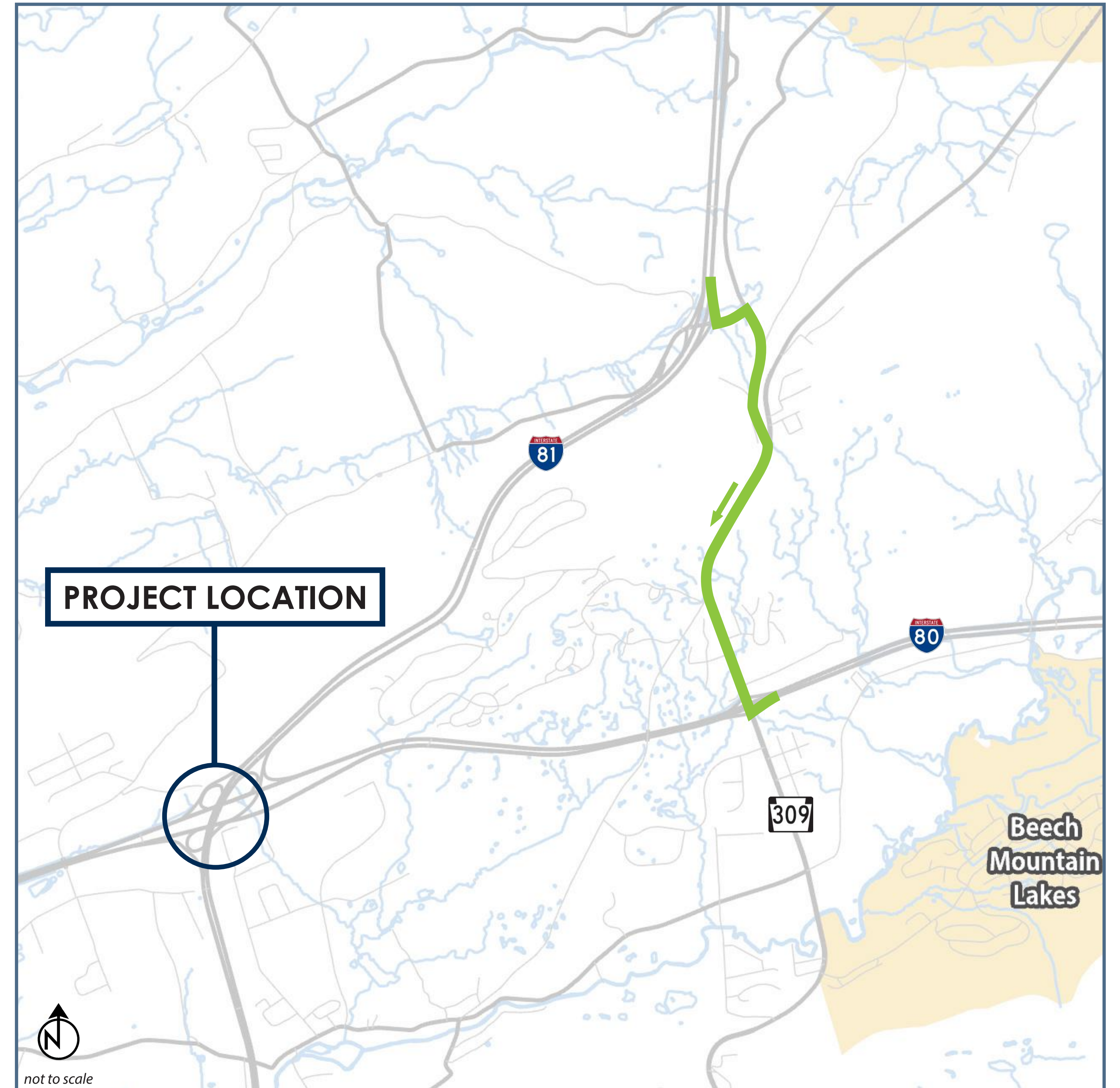
S.R. 8005 - Ramp C (S.R. 0081 Southbound to S.R. 0080 Eastbound) Long-term Ramp Detour (Stage 4) 3.1 miles
