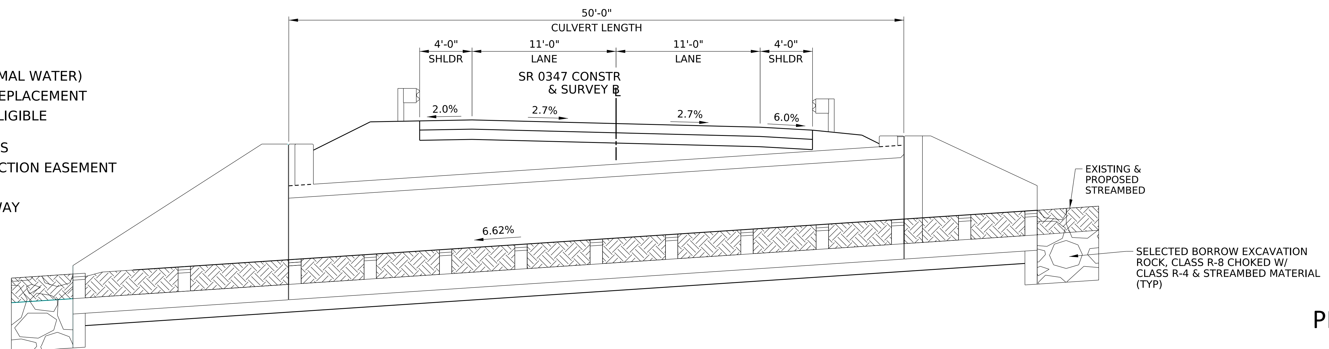
TYPICAL SECTION ALONG CULVERT
