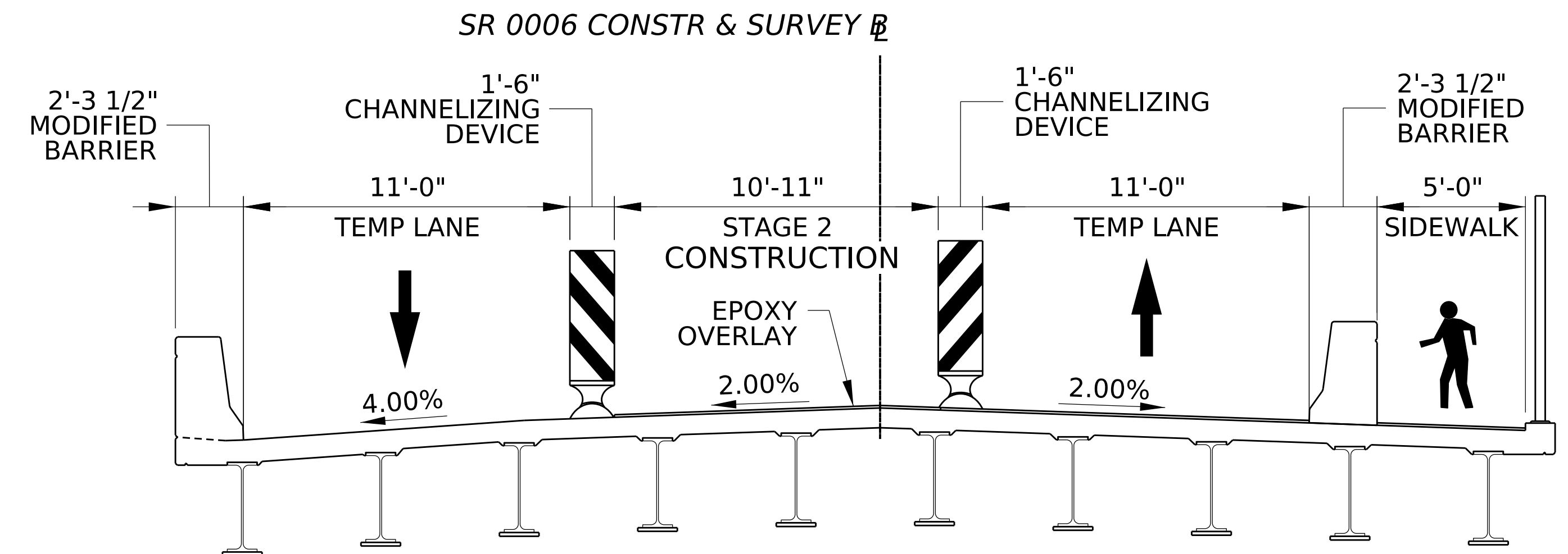
STAGE 2 TYPICAL SECTION
