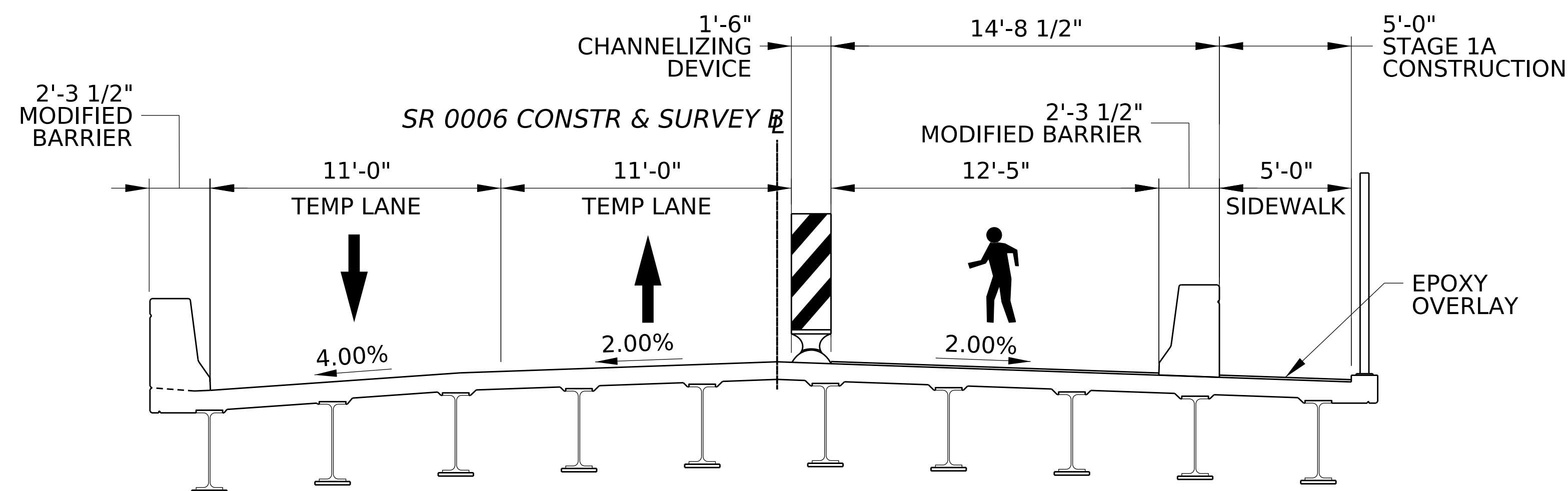
STAGE 1A TYPICAL SECTION
