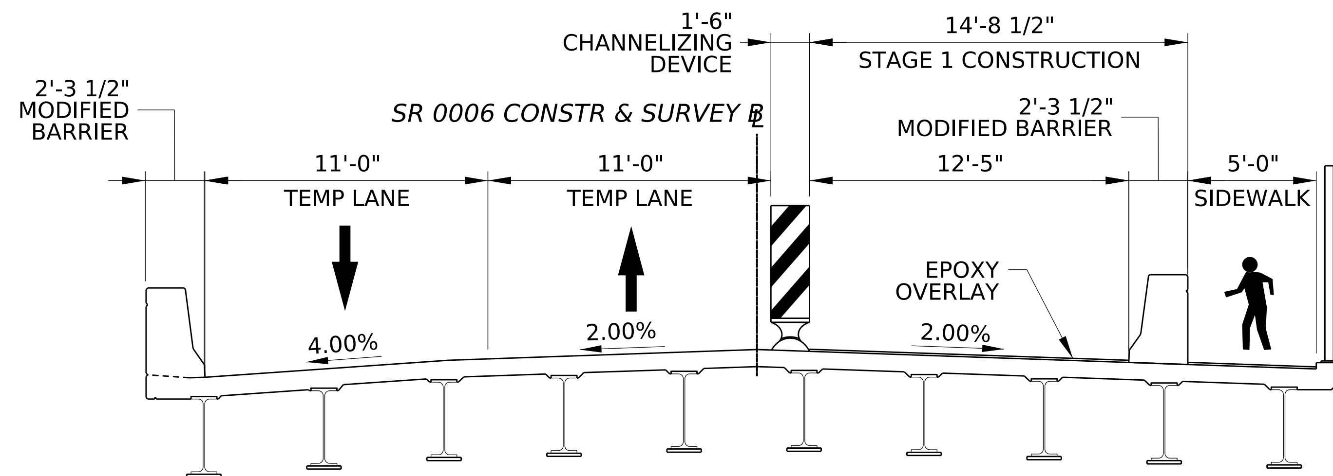
STAGE 1 TYPICAL SECTION
