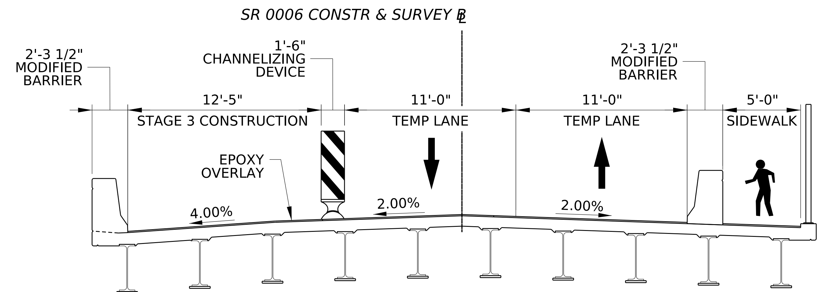
STAGE 3 TYPICAL SECTION
